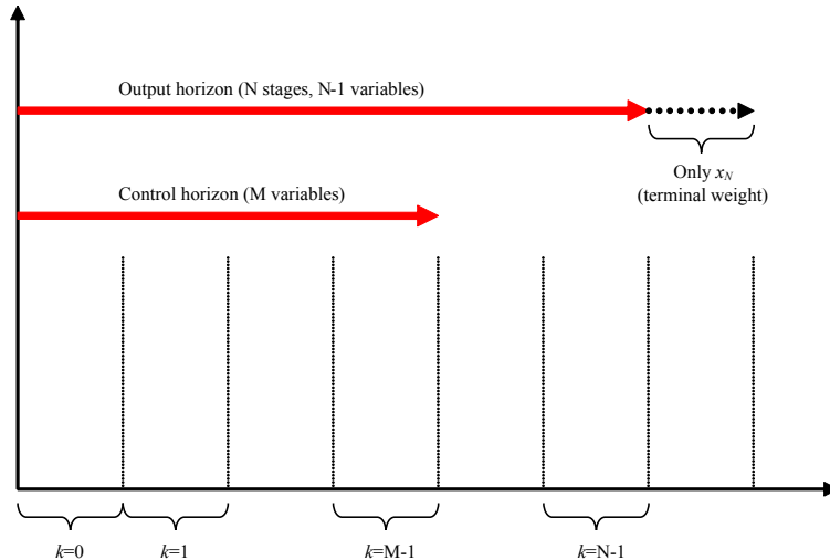
Figure 8: A schematic representation of the output and control horizon, OH and NC , respectively.
